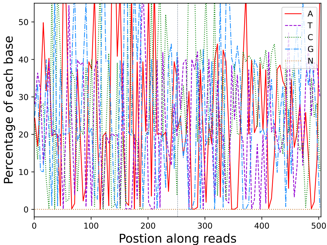
Base percentage along reads (R10621)
